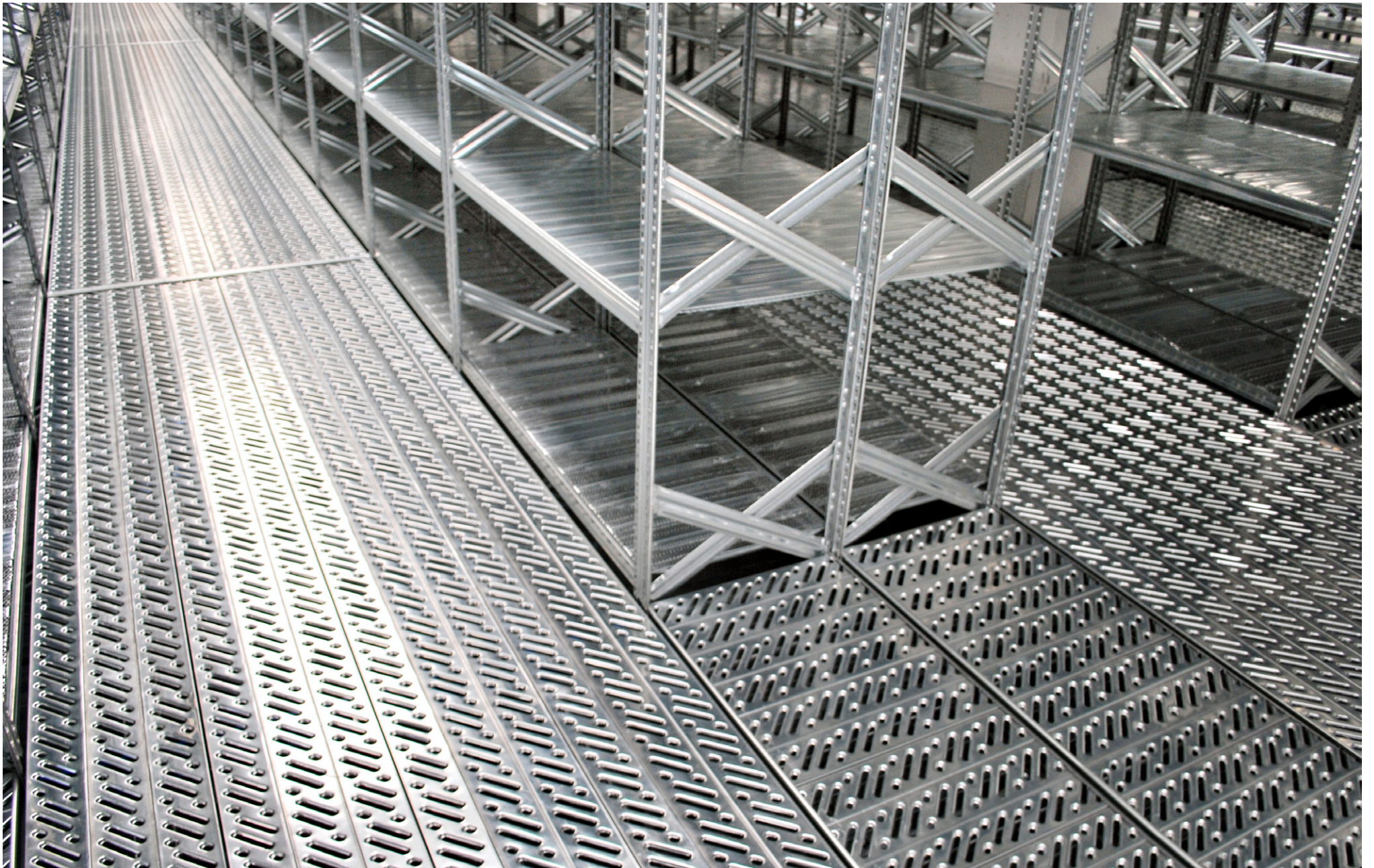
Super 1-2-3 Two-tier reference installation. <August 2013>
